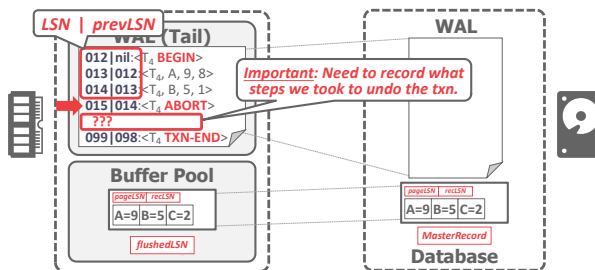
Figure 4: Transaction Abort – The DBMS maintains an LSN and prevLSN for each log record that the transaction creates. When the transaction aborts, all of the previous changes are reversed. After the log entries of the reversed changes make it to disk, the DBMS appends the TXN-END record to the log for the aborted transaction.
