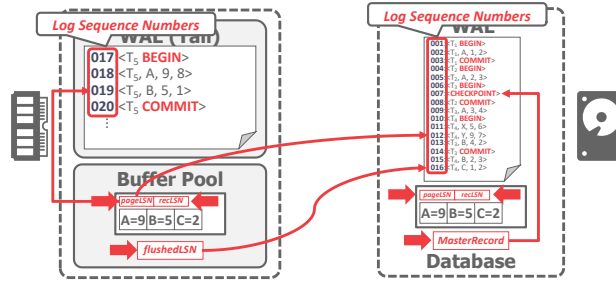
Figure 1: Writing Log Records – Each WAL has a counter of LSNs that is incremented at every step. The page also keeps a pageLSN and a recLSN, which stores the first log record that made the page dirty. The flushedLSN is a pointer to the last LSN that was written out to disk. The MasterRecord points to the last successful checkpoint passed.
